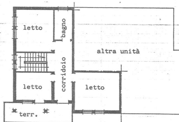
PIANO TERRA H=280
